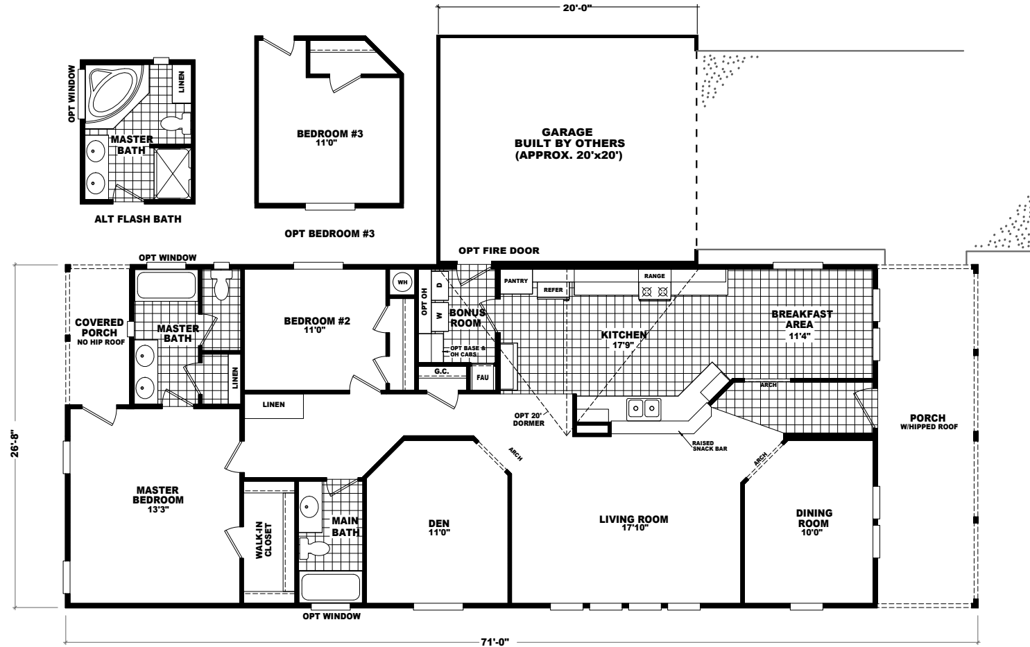
MODEL: 2871H APPROXIMATELY 1630 SQ. FT. 2 BEDROOM, 2 BATH SQUARE FOOTAGE DOES NOT INCLUDE PORCH
