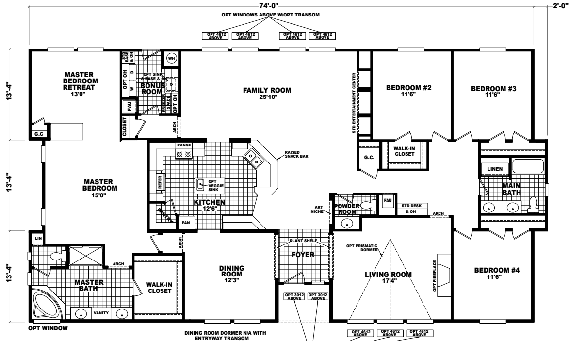
MODEL: 2918A APPROXIMATELY 2918 SQ. FT. 4 BEDROOM, 2 1/2 BATH
